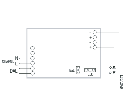
Non-maintained (emergency only) diagram
