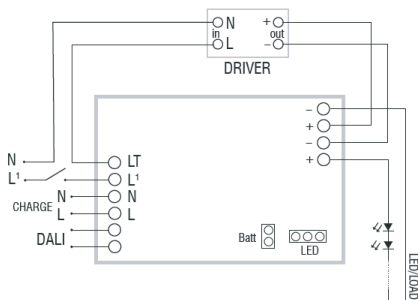
Maintained with external electronic driver diagram
